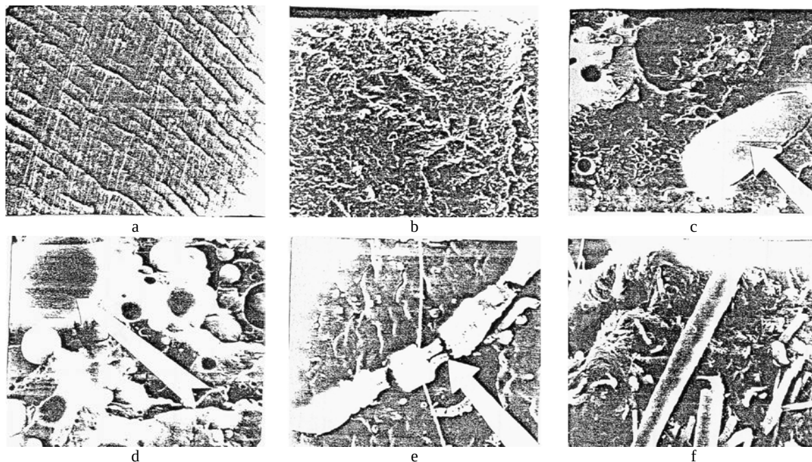
Figure 2 - The typical form of chips in liquid nitrogen (a-d) and fracture surfaces after uniaxial tension (d-f) samples from PA6 (a) SFD (b), the compositions PA6 + 5% wt. SFD (c, d) and PA6 + 50% by wt. SFD (e, f)
