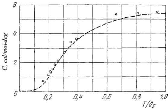
Figure 2 - The function C_V = f(T/\theta_D) in the P. Debye's theory of heat capacity [18]
