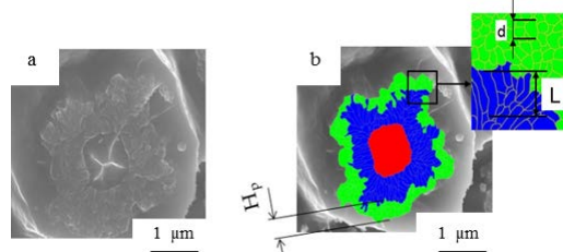
Fig. 3. Image of fracture: a - original of fracture surface; b - image after processing in AdobePhotoshopCS3 (TEM)
