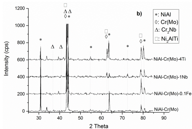
Fig. 3 XRD patterns of the alloys a) at room temperature and b) at high temperature.
