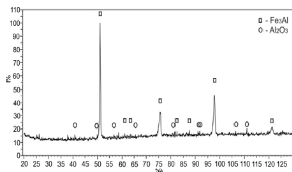
Fig. 1. X-ray diffraction pattern of a sample from a powder mixture \text{Fe} + 14\% \text{Al} after thermal synthesis and forging at a temperature of 1050^\circ\text{C}
