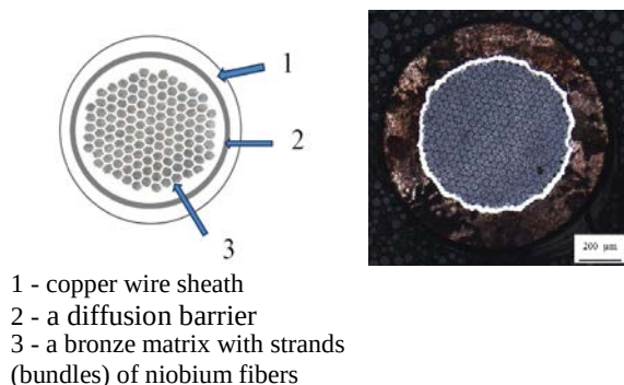
Fig. 1. Macrostructure of superconductors
