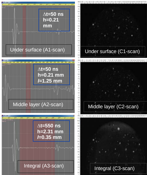
Fig.3 Acoustic waveforms (A-scans) and images (C-scans) of the specimen S50-2.
