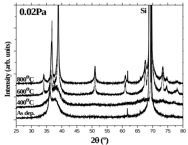
Fig. 3 The diffraction patterns for the sample deposited with P(\text{N}_2 + \text{O}_2) = 0.02 \text{ Pa} , obtained for the as deposited film, and for the 400^\circ\text{C} , 600^\circ\text{C} and 800^\circ\text{C} annealed films.
