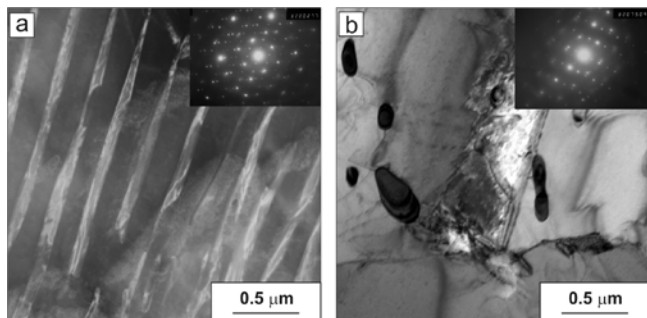
Fig. 1. The microstructure of the steel in the initial nitrided state (TEM): a - condition 1; b - condition 2
