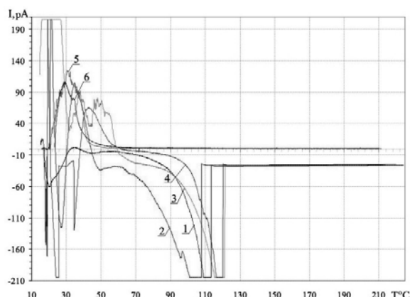
Figure 3 Characteristic form TSC-spectrum shungite source (1) and heat-treated at 100 °C (2) 200 °C (3) 300 °C (4), 600 °C (5) 800 °C (6)
