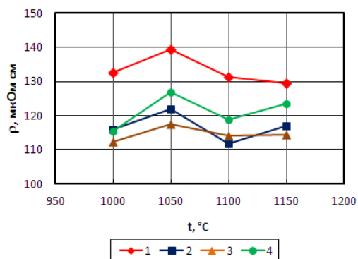
Fig. 4. Relationship between electrical resistivity and forging temperature for the samples after: 1 – hot forging (HF); 2 – hot forging + sintering at 1100^\circ\text{C} ; 3 – forging + sintering at 1300^\circ\text{C} ; 4 – forging + sintering at 1450^\circ\text{C}
