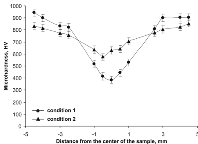
Fig. 3. The distribution of the microhardness of the diameter of the sample after the HPT
