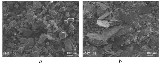
Fig. 8. The morphology of initial powder mixtures after mixing in a tumbling mixer (a) and milling in a planetary mill (b)
