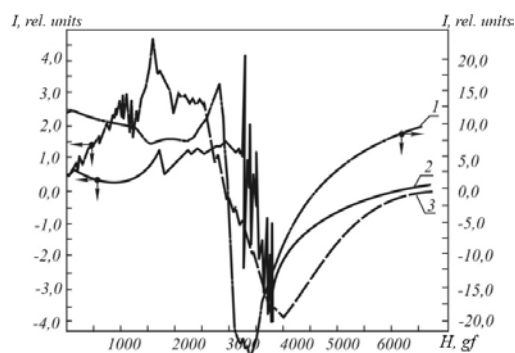
Figure 2 EPR spectra of opal (1) and clay minerals of different composition (2, 3)
