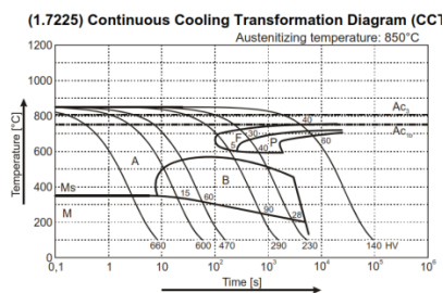
Figure 8 Diagram of continous cooling (CCT) for 42CrMo4 steel [9]
