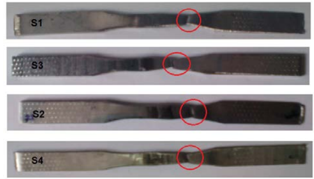
Fig.6 Broken specimens
