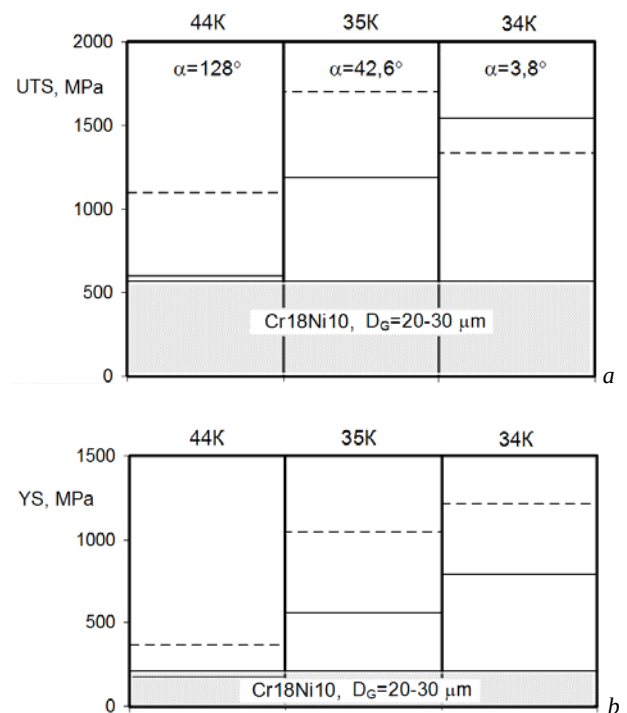
Fig. 1. Comparison of calculated (solid lines) and experimental (dashed) values of strength UTS (a) and YS (b) for alloys 44K, 35K and 34K and traditional corrosion-resistant austenitic steel Cr18Ni10 [6]
