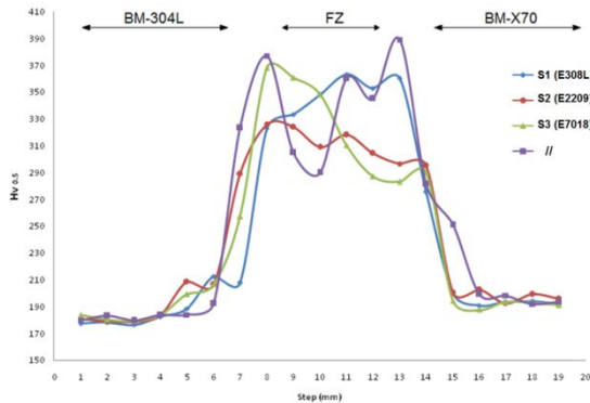
Fig.5 Microhardness profiles
