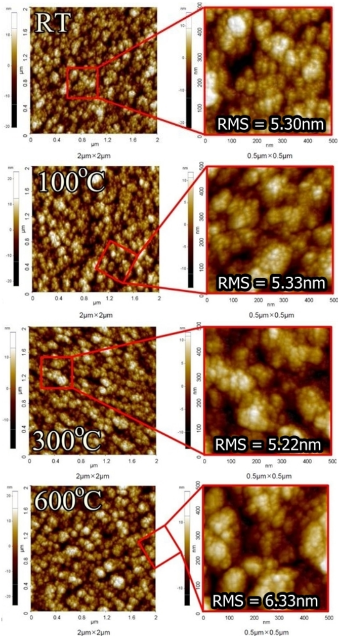
Fig. 5 The influence of temperature on the surface roughness, for the sample obtained with P(N_2 + O_2) = 0.02 Pa.
