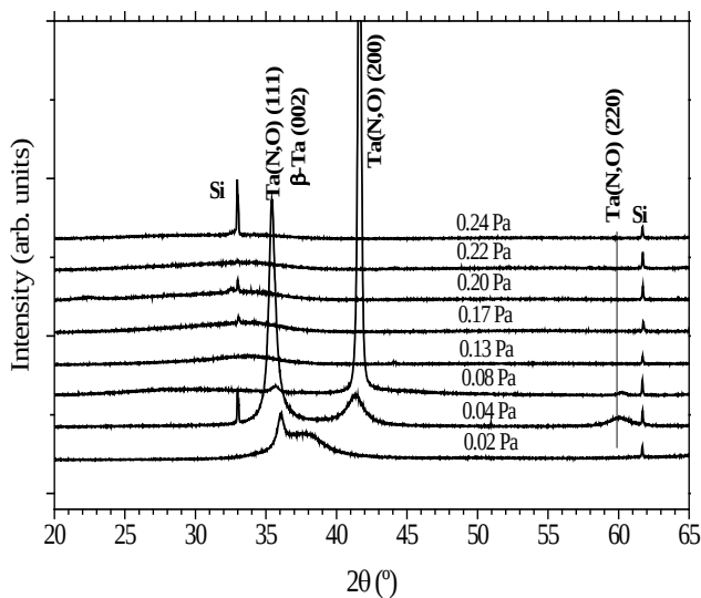
Fig. 2 X-Ray diffraction patterns, as a function of the reactive gas partial pressure, for the tantalum oxynitride films (Si – substrate, silicon).
