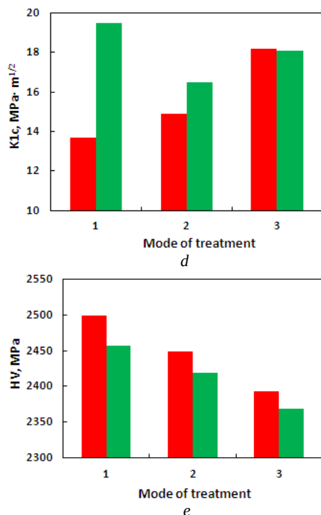
Fig. 9. The effect of processing modes and type of original powder mixture on density (a) and the basic physical and mechanical properties (b-e) of intermetallics
