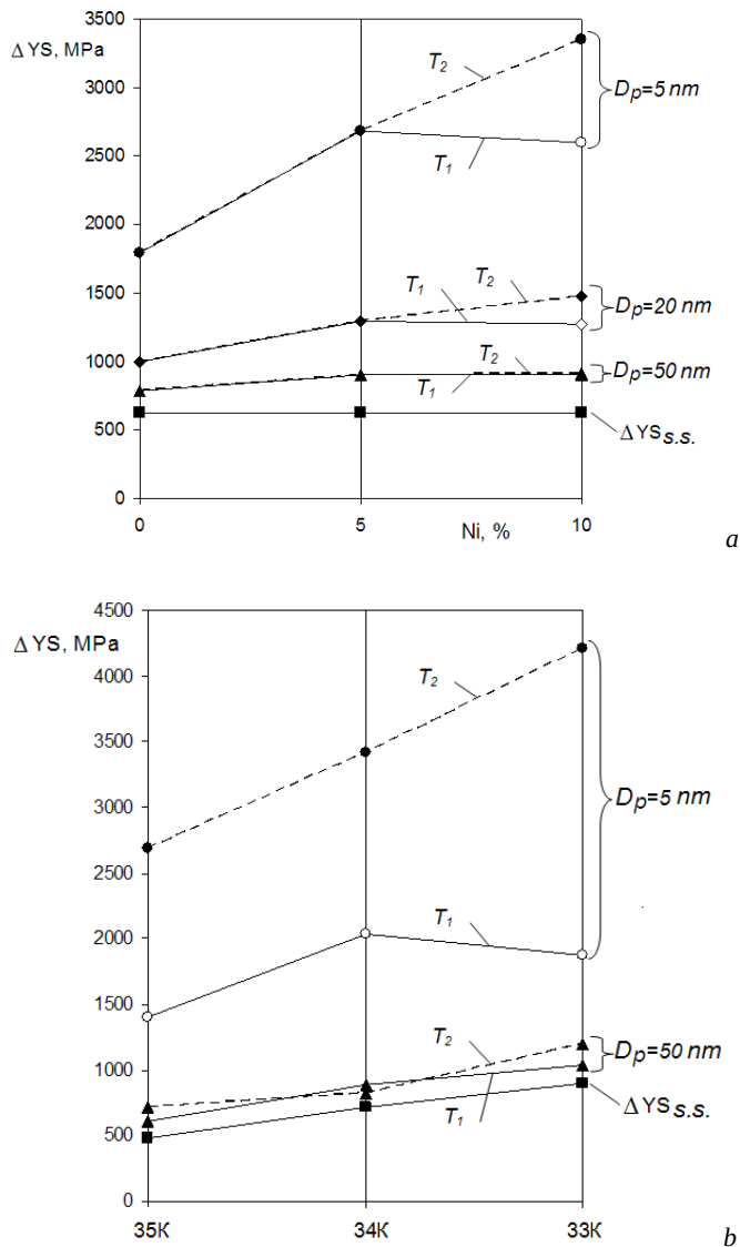
Fig 2. The growth of values alloy yield strength \Delta YS Fe-20%Mn-10%Al-1.4%C-x%Ni (a) and experimental alloys (b) due to aging at different temperatures ( T_1 and T_2 denote as in tables 2 and 3) and obtain different particle size D_p
