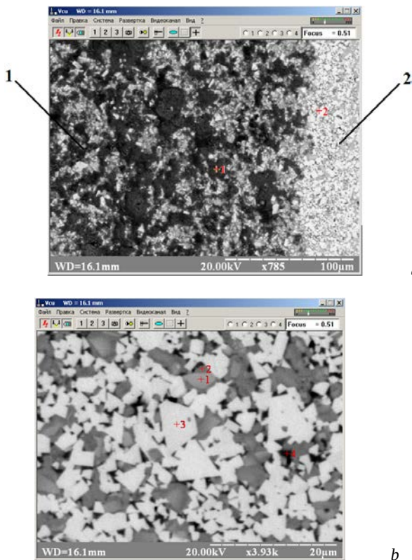
Fig.2: Surface topography (a - (1 – surface (surface area 1 is at an angle of 18° from the subsurface zone, 2) 2 – subsurface zone); chemical analysis determined the points +1, +2) and the structure of the surface area (b – chemical analysis determined the points +1, +2, +3, +4) hard alloys T15K6 with boride coating obtained at introduction of the saturating powder environment \text{Cu}_2\text{O}
