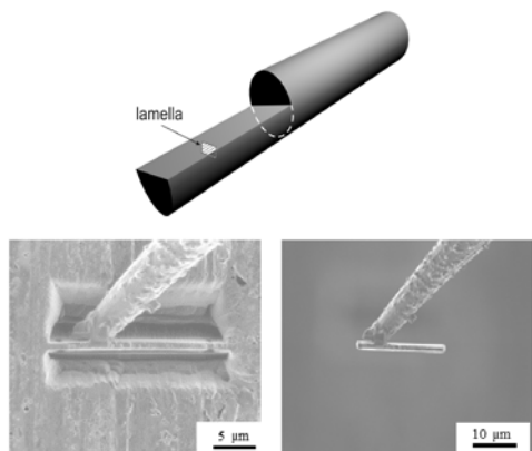
Fig. 4. The main stages of sample preparation for TEM studies
