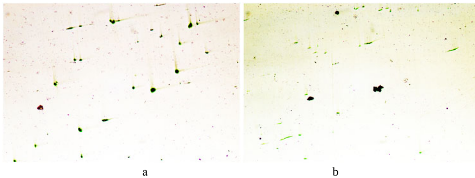
Figure 2 (a and b) Non metallic inclusions present in the investigated specimen, x100
