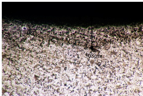
Figure 4 Microstructure of induction quenched layer, x100, Kalings reagent
