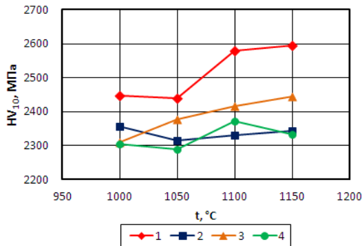
Fig. 7. Relationship between hardness and forging temperature for the samples after: 1 – hot forging (HF); 2 – hot forging + sintering at 1100 \text{ }^\circ\text{C} ; 3 – forging + sintering at 1300 \text{ }^\circ\text{C} , 4 – forging + sintering at 1450 \text{ }^\circ\text{C}
