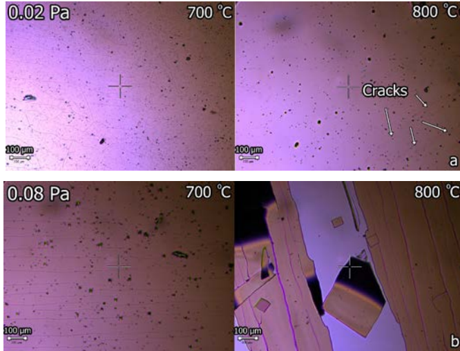
Fig. 4 Failure features observed on the surface of the annealed samples, deposited with P(N_2 + O_2) = 0.02 Pa (a) and P(N_2 + O_2) = 0.08 Pa (b).
