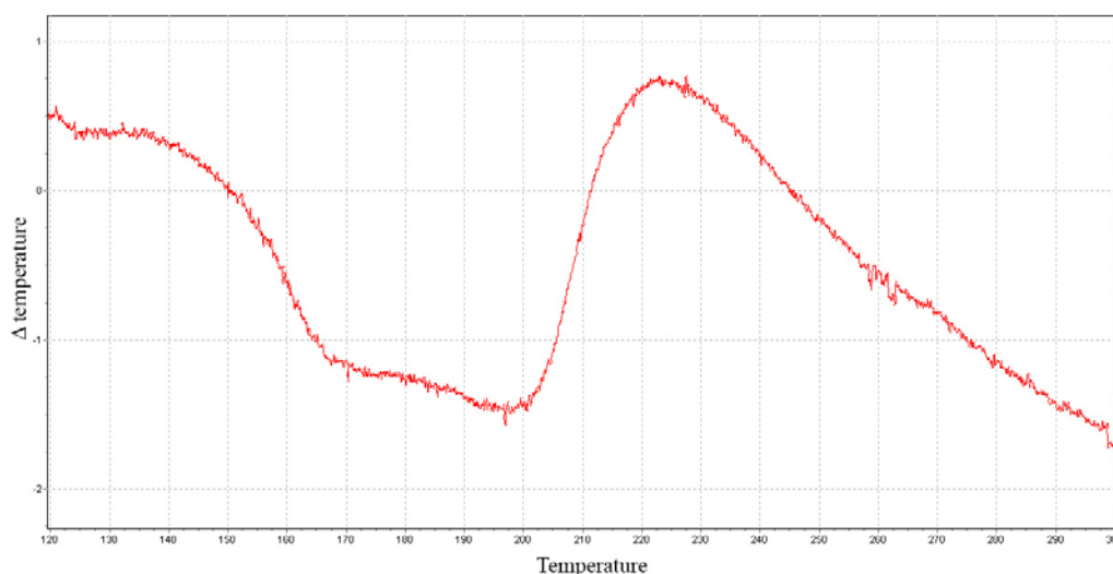
Figure 3 - DTA curve of polypropylene subjected to recycling
