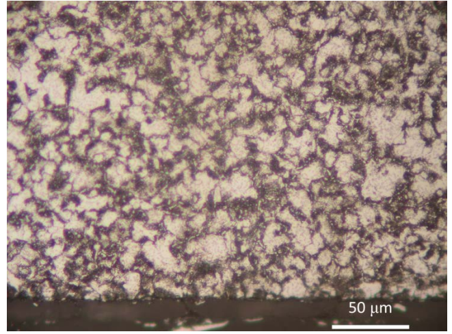
Fig. 2. Carburized surface of steel 40X13 specimen
