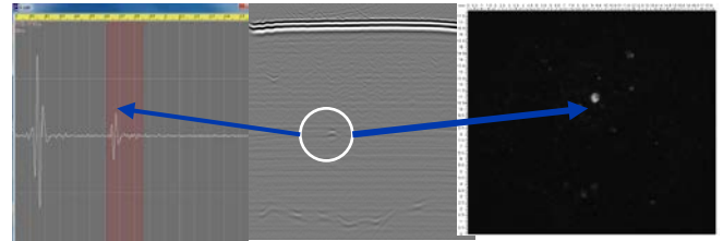
Fig. 5 Acoustic waveforms (A-scans) and images (B- and C-scans) of a sample of c-BN/C 60 . The kind of reflection from the bottom of the sample on the B-scan indicates its great heterogeneity.
