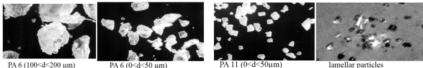
Figure 4 - The characteristic morphology of the particulate fraction of nanocomposites based on PA 6 and PA 11
