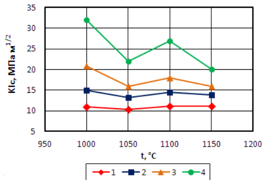
Fig. 6. Relationship between bending fracture toughness and forging temperature for the samples after: 1 – hot forging (HF); 2 – hot forging + sintering at 1100 \text{ }^\circ\text{C} ; 3 – forging + sintering at 1300 \text{ }^\circ\text{C} , 4 – forging + sintering at 1450 \text{ }^\circ\text{C}
