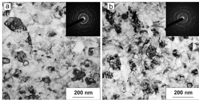
Fig. 4. The microstructure of the steel after HPT and annealing at 450 °C (TEM): a - condition 1; b - condition 2
