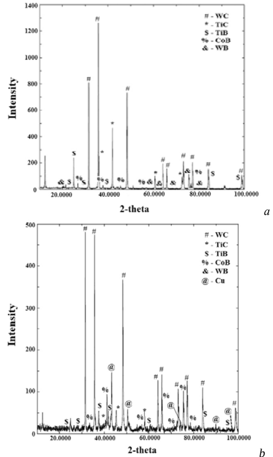
Fig.3: Diffractograms taken from the surface of hard alloys T15K6 with boride coatings in \text{Cu K}\alpha_1, \text{K}\alpha_2 monochromatic radiation: a – coating after boriding; b – coating after complex saturation with boron and copper in the environment with the addition copper containing powder \text{Cu}_2\text{O} , diffraction peaks of Cu line (111), (200), (220), (311), (222)
