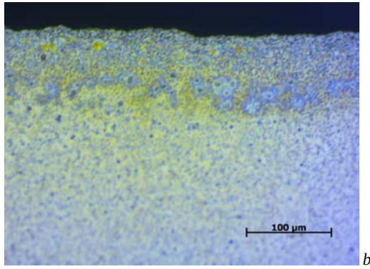
Fig.1: Microstructures boride coatings on hard alloys T15K6: a – coatinga after boriding, 4 hours, x200; b – after complex saturation with boron and copper, 4 hours, x200
