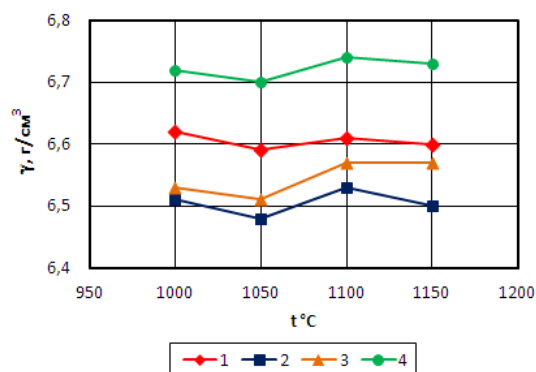
Fig. 2. Relationship between materials density and forging temperature for the samples after: 1 – hot forging (HF); 2 – hot forging + sintering at 1100^\circ\text{C} ; 3 – forging + sintering at 1300^\circ\text{C} ; 4 – forging + sintering at 1450^\circ\text{C}
