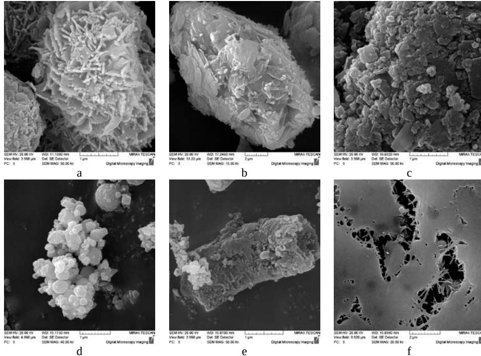
Figure 4 - A typical particle morphology tripoli (a), clay (b), shungite (c) metal oxide (d), carbon nanotubes (e), polytetrafluoroethylene (f)
