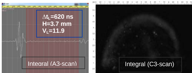
Fig. 4 Acoustic waveforms (A-scans) and images (C-scans) of the specimen S10-5.
