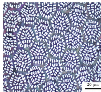
Fig.2. Microstructure of superconductors (SEM)
