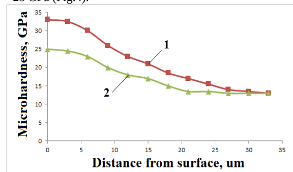
Fig.4: Microhardness boride coating: 1 – coating after boriding; 2 – coating after complex saturation with boron and copper
