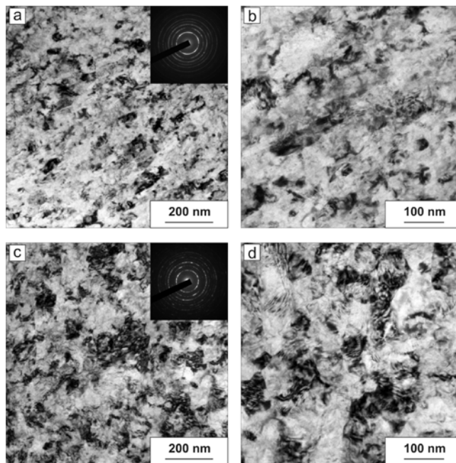
Fig. 2. The microstructure of the steel after HPT (TEM): a, b - condition 1; c, d - condition 2
