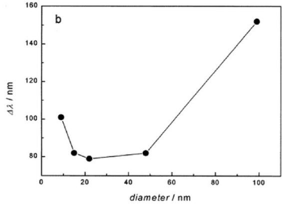
Figure 3 - Dependence of the maximum width of the plasmon ( \Delta\lambda ) on the diameter of the spherical gold nanoparticle [5]
