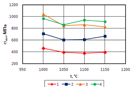
Fig. 5. Relationship between bending strength and forging temperature for the samples after: 1 – hot forging (HF); 2 – hot forging + sintering at 1100^\circ\text{C} ; 3 – forging + sintering at 1300^\circ\text{C} ; 4 – forging + sintering at 1450^\circ\text{C}
