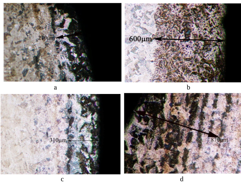
Figure 6 (a-d) Microstructure surface (quenched layer) at different positions of specimen
