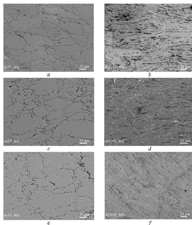
Fig. 10. The structure of the mixture intermetallic compounds I (a, c, e) and II (b, d, f) after hot forging (a, b) and subsequent annealing at 1100 °C (c, d) and 1300 °C (e, f)
