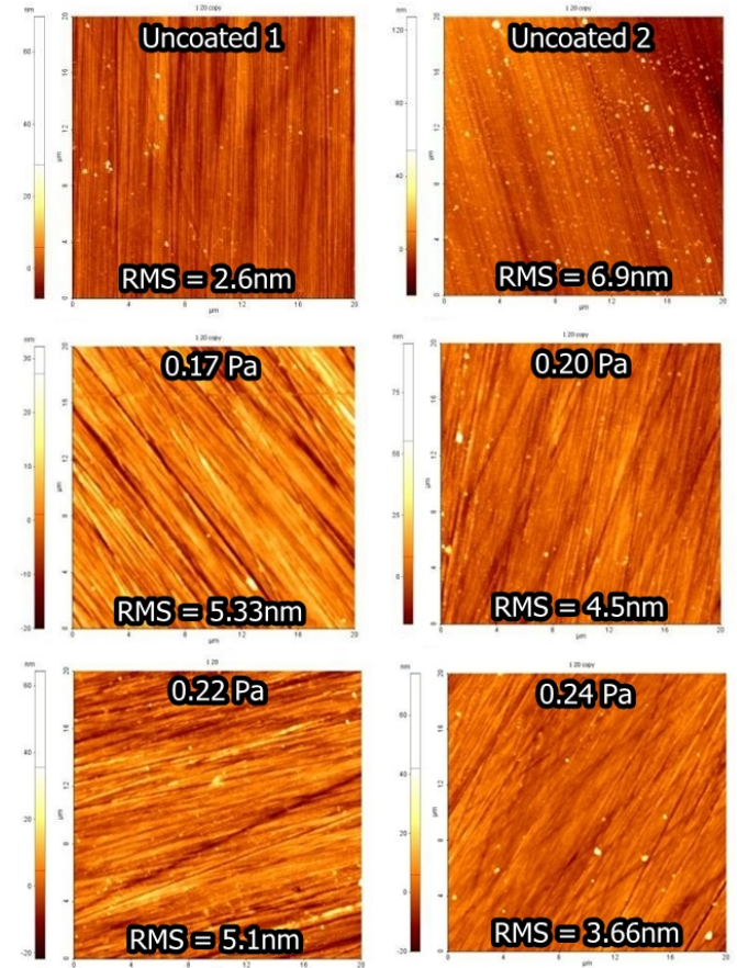
Fig. 5 AFM micrographs obtained from uncoated substrates and from the intermediate and high partial pressure samples (a,b – uncoated, c – P(N_2 + O_2) = 0.17 Pa, d – P(N_2 + O_2) = 0.20 Pa, e – P(N_2 + O_2) = 0.22 Pa, f – P(N_2 + O_2) = 0.24 Pa).
