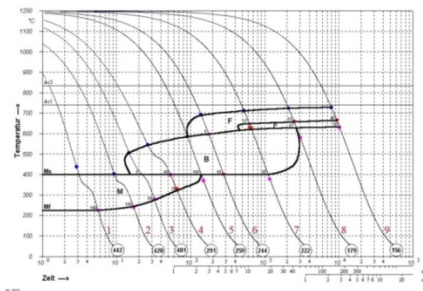
Figure 9 Diagram of continous cooling (CCT) for 16MnCr5 steel [10]
