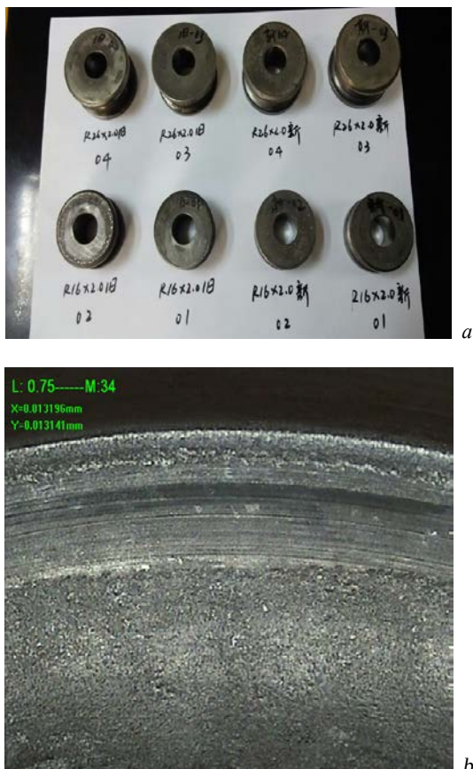
Fig.5: Rollers (a) and topography surface wear coating on the rollers(b)
