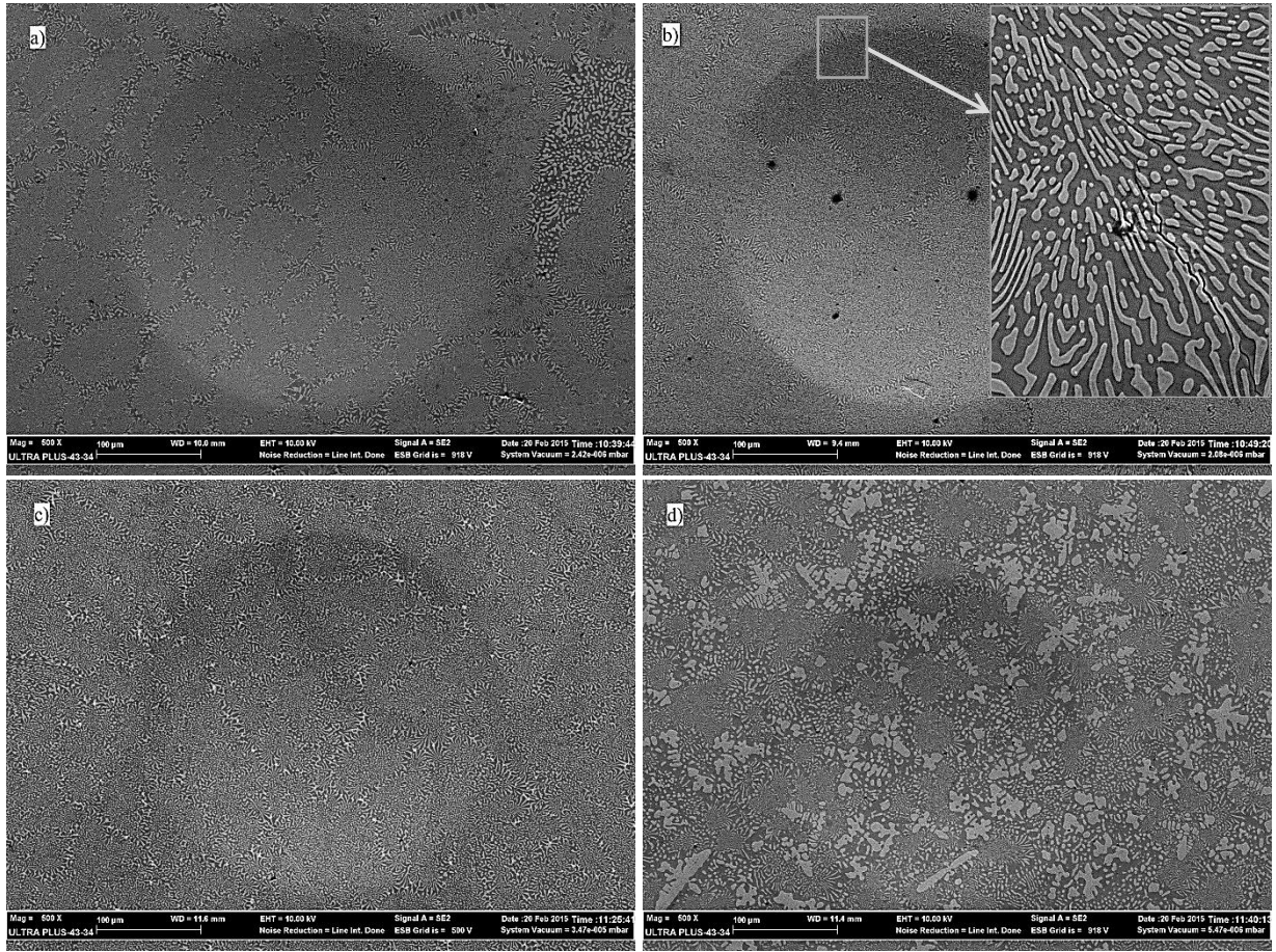
Fig. 4 Deformations on the indentation for; a) NiAl-Cr(Mo), b) NiAl-Cr(Mo)-0.1Fe, c) NiAl-Cr(Mo)-1Nb and d) NiAl-Cr(Mo)-4Ti.
