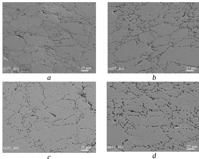
Fig. 3. The structure of the samples after forging at 1100^\circ\text{C} (a) and subsequent sintering at 1100^\circ\text{C} (b); 1300^\circ\text{C} (c) and 1450^\circ\text{C} (d)
