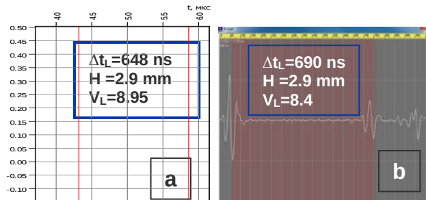
Fig.2 The waveforms of ultrasonic pulses of the specimen S50-2 obtained by the laser optoacoustic method (a) and the acoustic microscopy method (b). ( \Delta t_L - time-of-flight double thickness H of the specimen)
