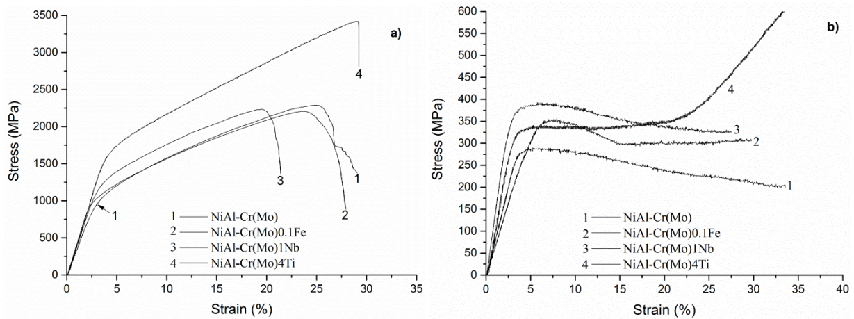
Fig. 5. Compression stress-strain curves, a) at room temperature and b) at 1000°C.
